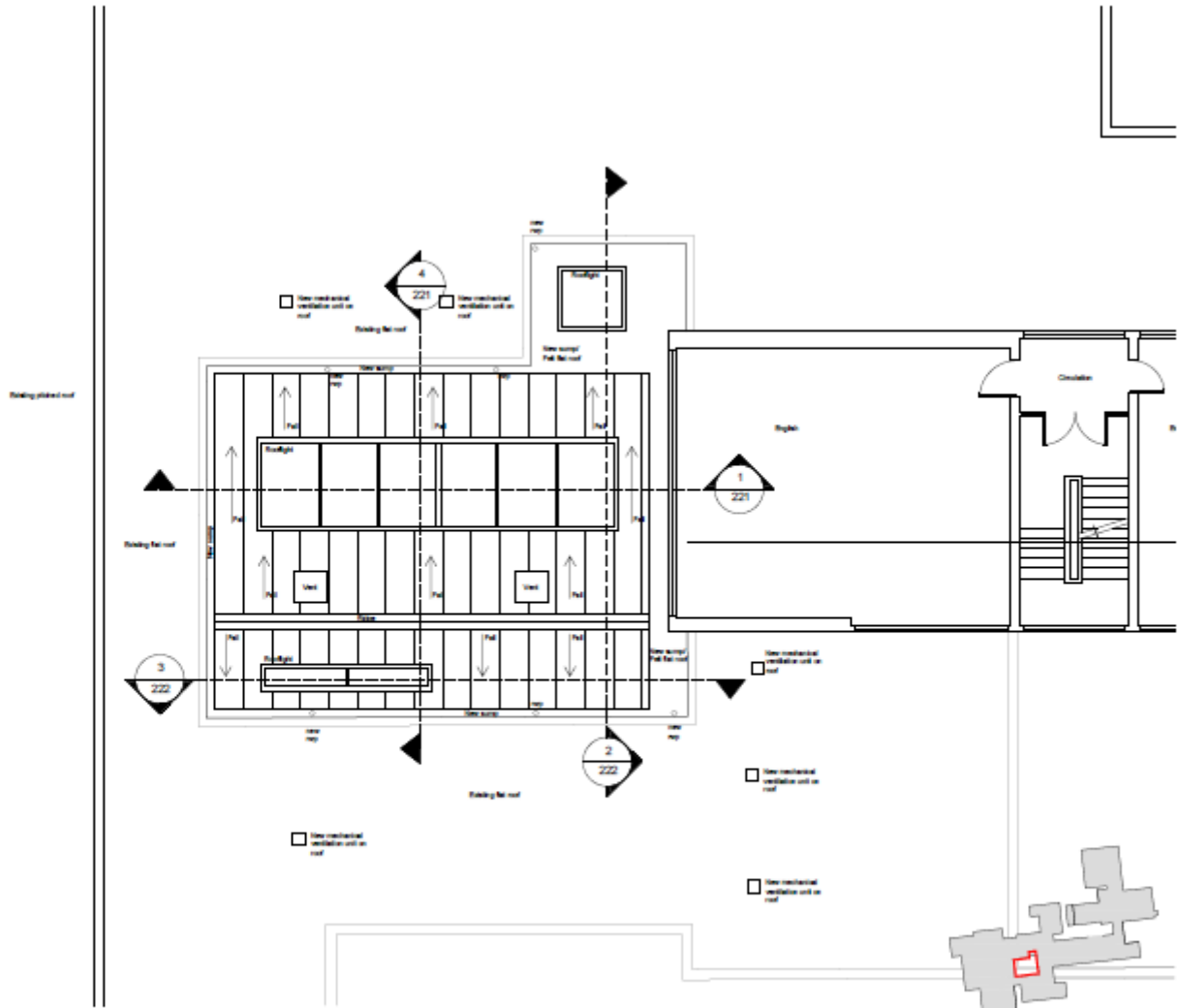
Quadrangle courtyard Roof level plan - Proposal
